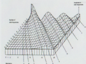
Figure 4.13 Three-dimensional graph of the Bessel functions J_0 to J_{12} plotted (plotted back to front) as a function of modulation index J (plotted from left to right) showing the number of sidebands generated (after Chowning 1977). Lines A, B, and C show the points at which the amplitude falls off by -40, -60, and -80 dB, respectively. Line D indicates the cutoff point for "perceptually significant" sidebands. E is the maximum amplitude for each order. Lines F through K show the zero-crossings of the functions and, therefore, values of the index that produce a null or zero amplitude for various side frequencies.
